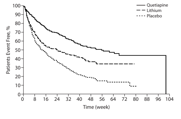
Figure 4. Time to All-Cause Discontinuation (Kaplan-Meier curves, ITT population)
